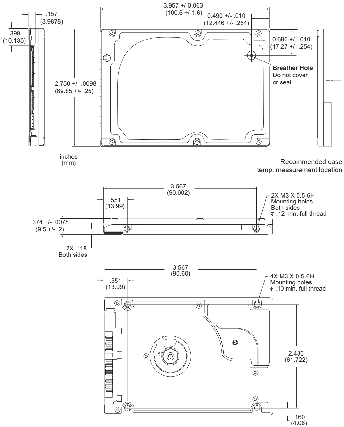
Figure 4. Mounting dimensions—top, side and end view
