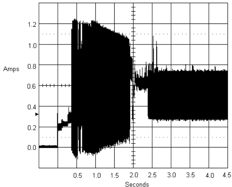
Figure 1. Typical 5V startup and operating current profile
