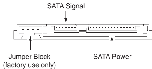
Figure 2. Serial ATA connectors
